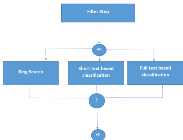
Figure 1: Proposed Approach
